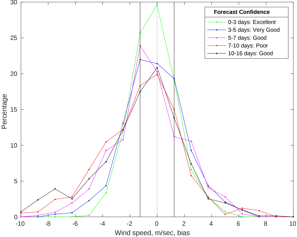
NDBC 46054 vs GFS Winds Bias Histogram: 22-Jun-2025
