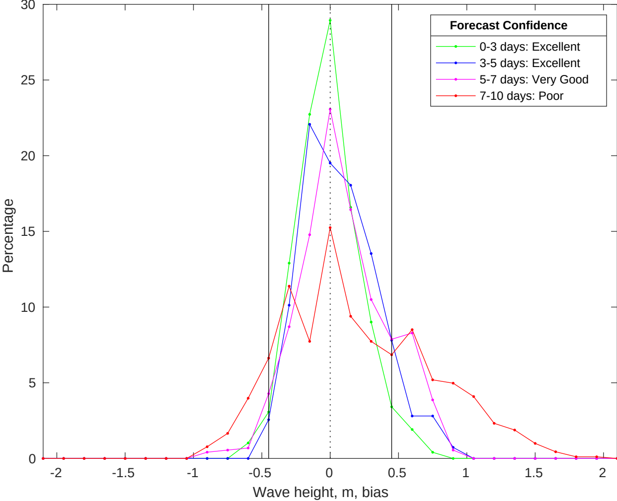
NDBC 46069 vs CMEMS Waves Bias Histogram: 22-Jun-2025
