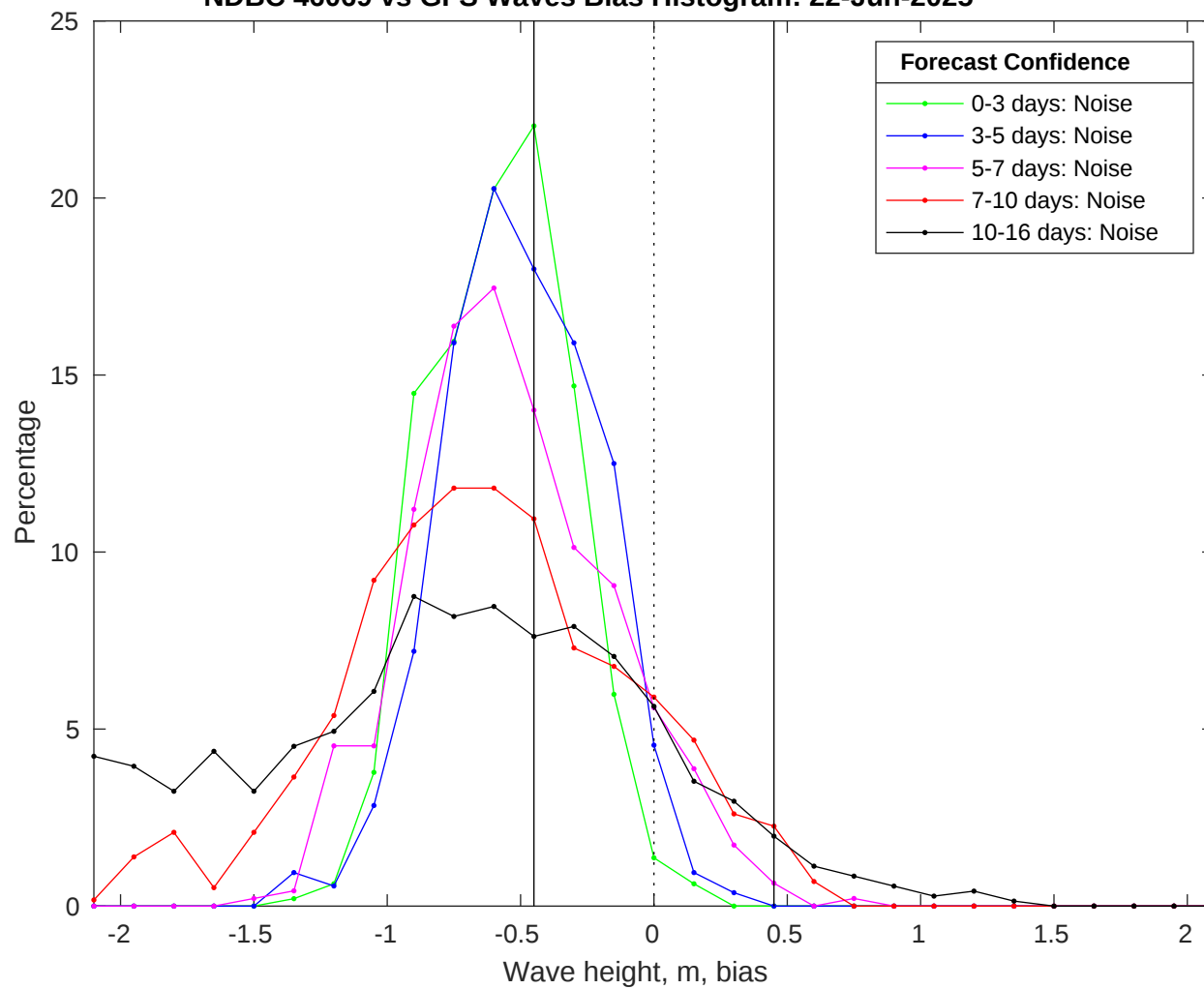
NDBC 46069 vs GFS Waves Bias Histogram: 22-Jun-2025
