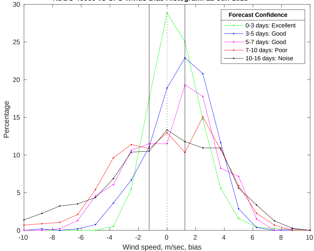
NDBC 46069 vs GFS Winds Bias Histogram: 22-Jun-2025
