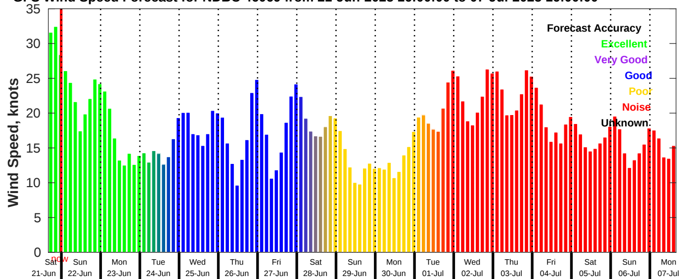
GFS Wind Speed Forecast for NDBC 46069 from 21-Jun-2025 16:00:00 to 07-Jul-2025 16:00:00
