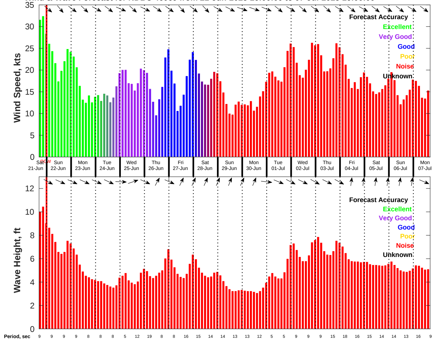
Wind & Wave Forecast for NDBC 46069 from 21-Jun-2025 16:00:00 to 07-Jul-2025 16:00:00
