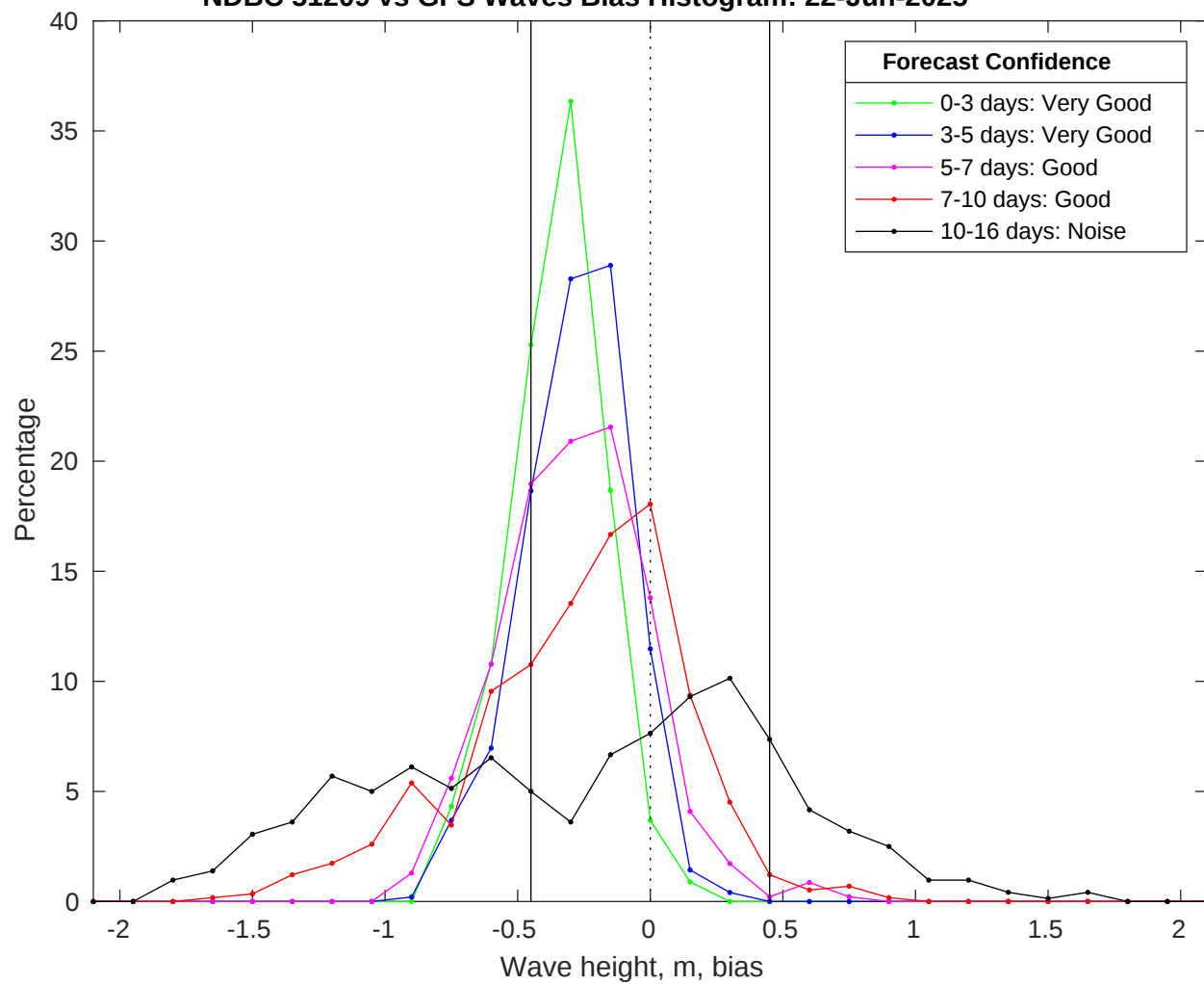
NDBC 51209 vs GFS Waves Bias Histogram: 22-Jun-2025
