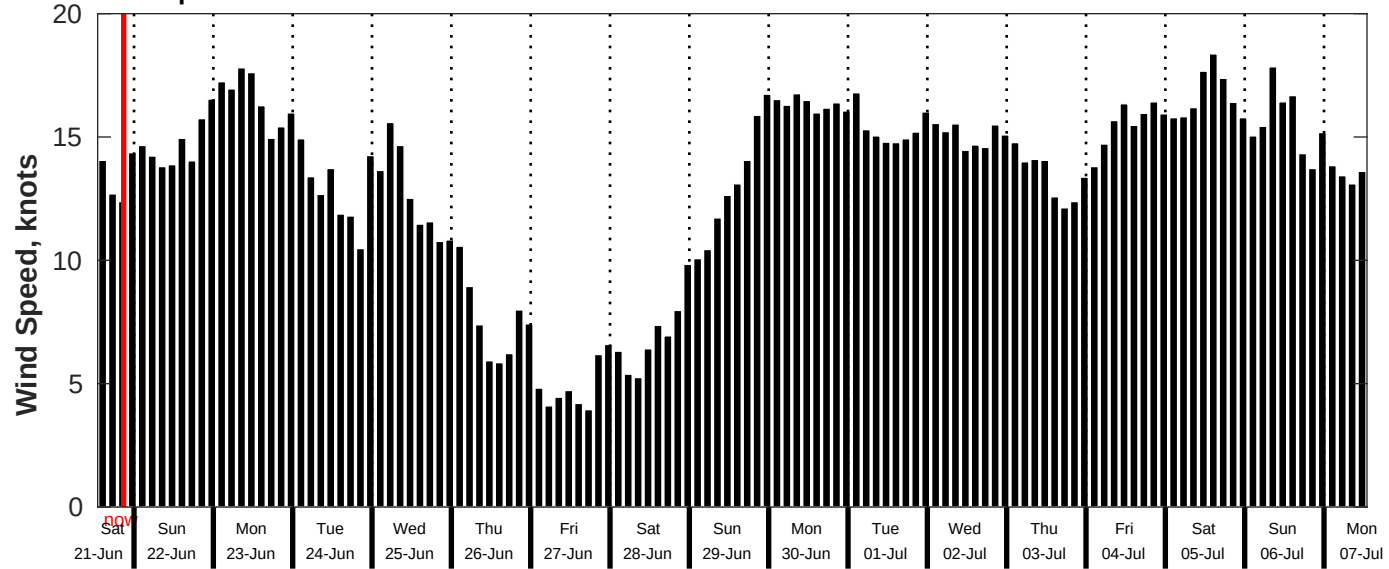
GFS Wind Speed Forecast for NDBC 51209 from 21-Jun-2025 13:00:00 to 07-Jul-2025 13:00:00
