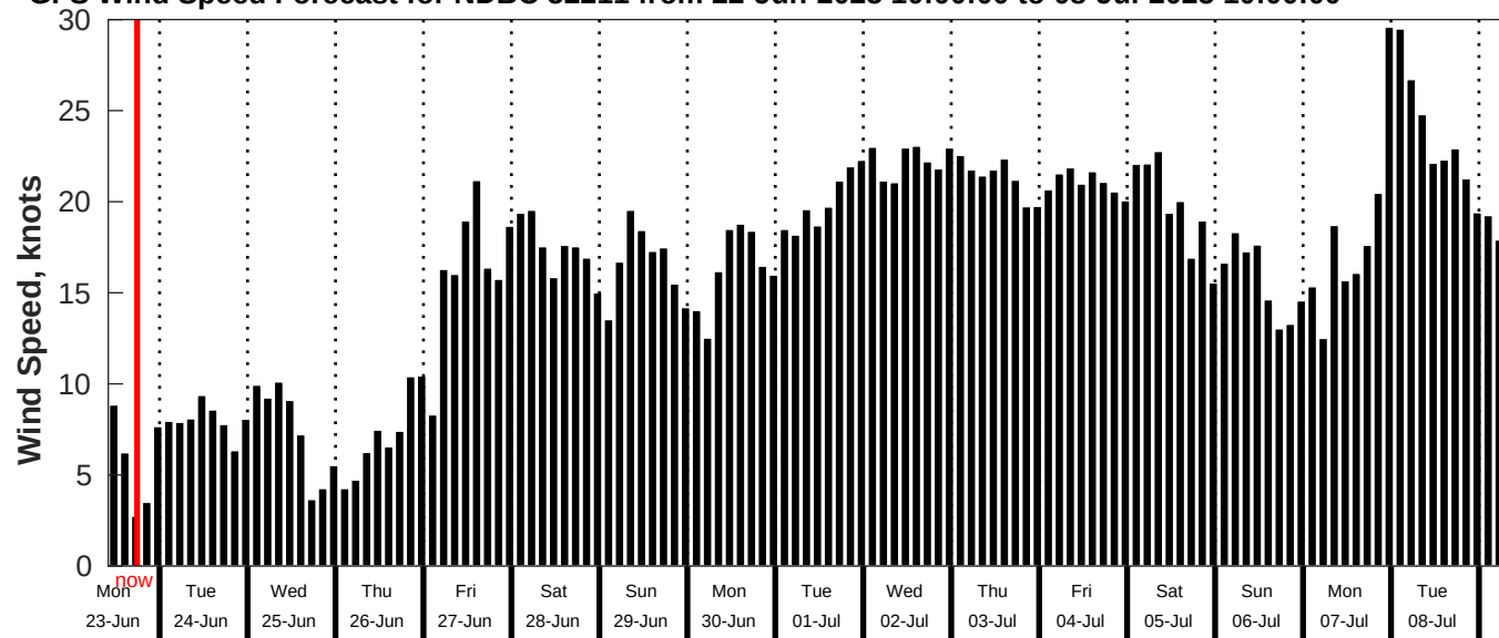
GFS Wind Speed Forecast for NDBC 52211 from 22-Jun-2025 10:00:00 to 08-Jul-2025 10:00:00
