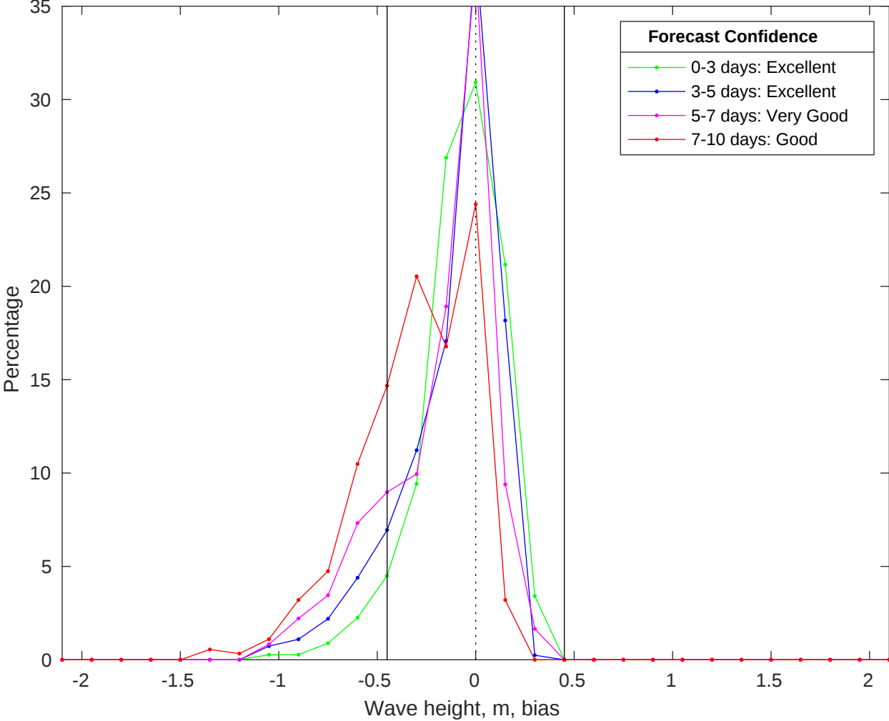
NDBC 52212 vs CMEMS Waves Bias Histogram: 22-Jun-2025
