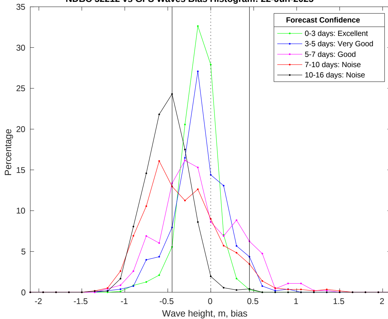
NDBC 52212 vs GFS Waves Bias Histogram: 22-Jun-2025
