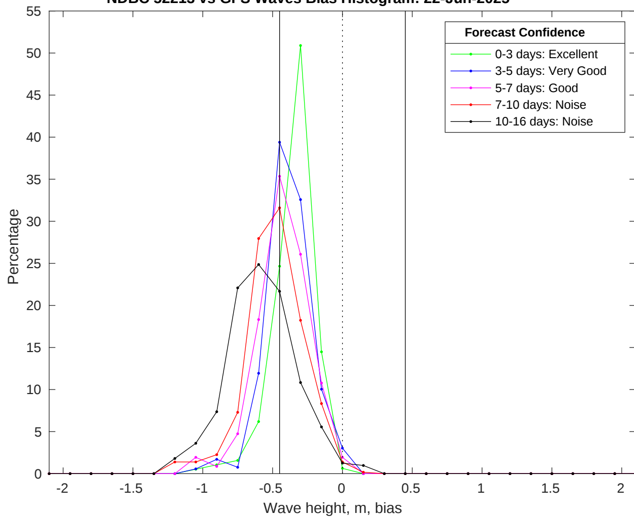
NDBC 52213 vs GFS Waves Bias Histogram: 22-Jun-2025
