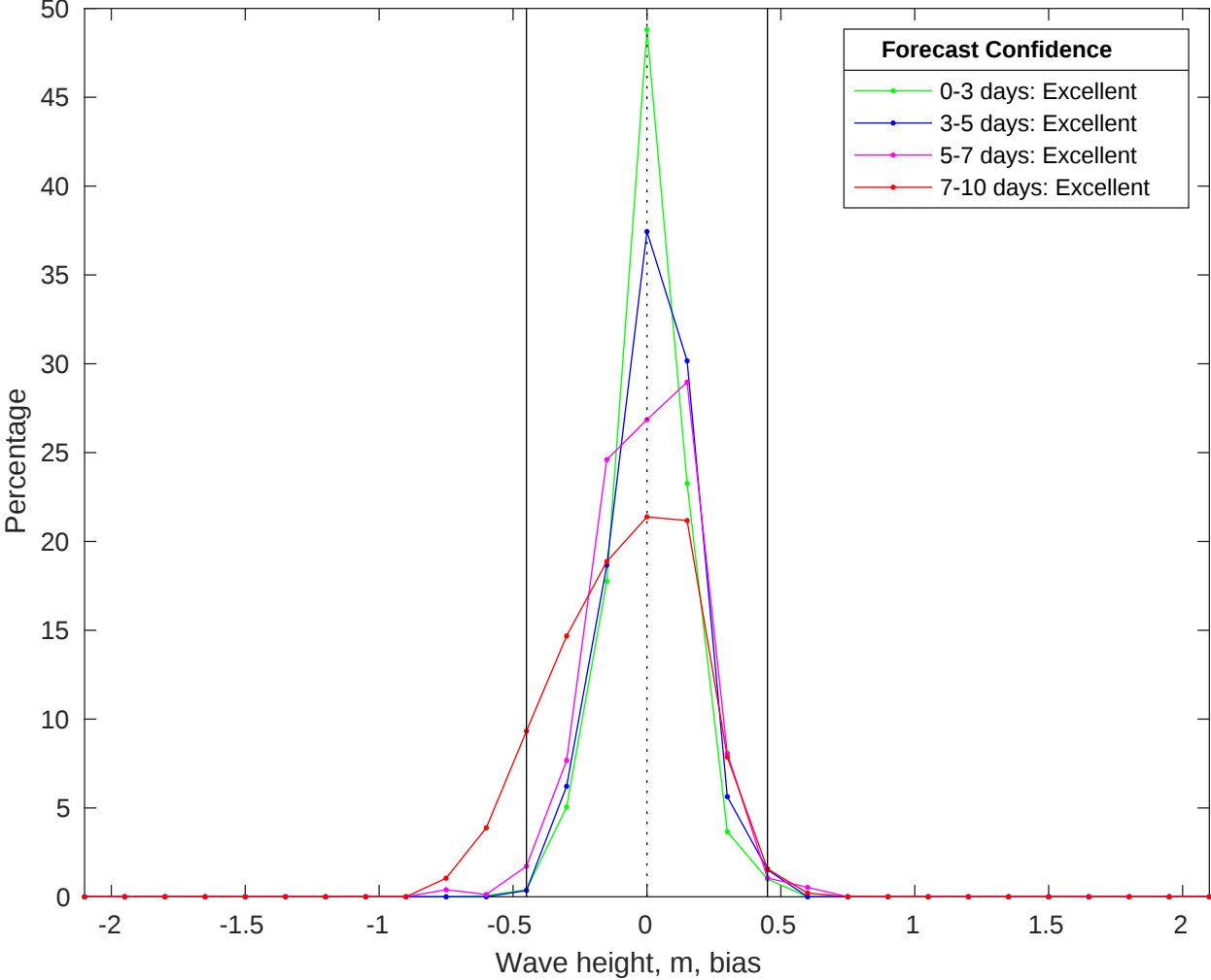
NDBC 41004 vs CMEMS Waves Bias Histogram: 23-Jun-2025
