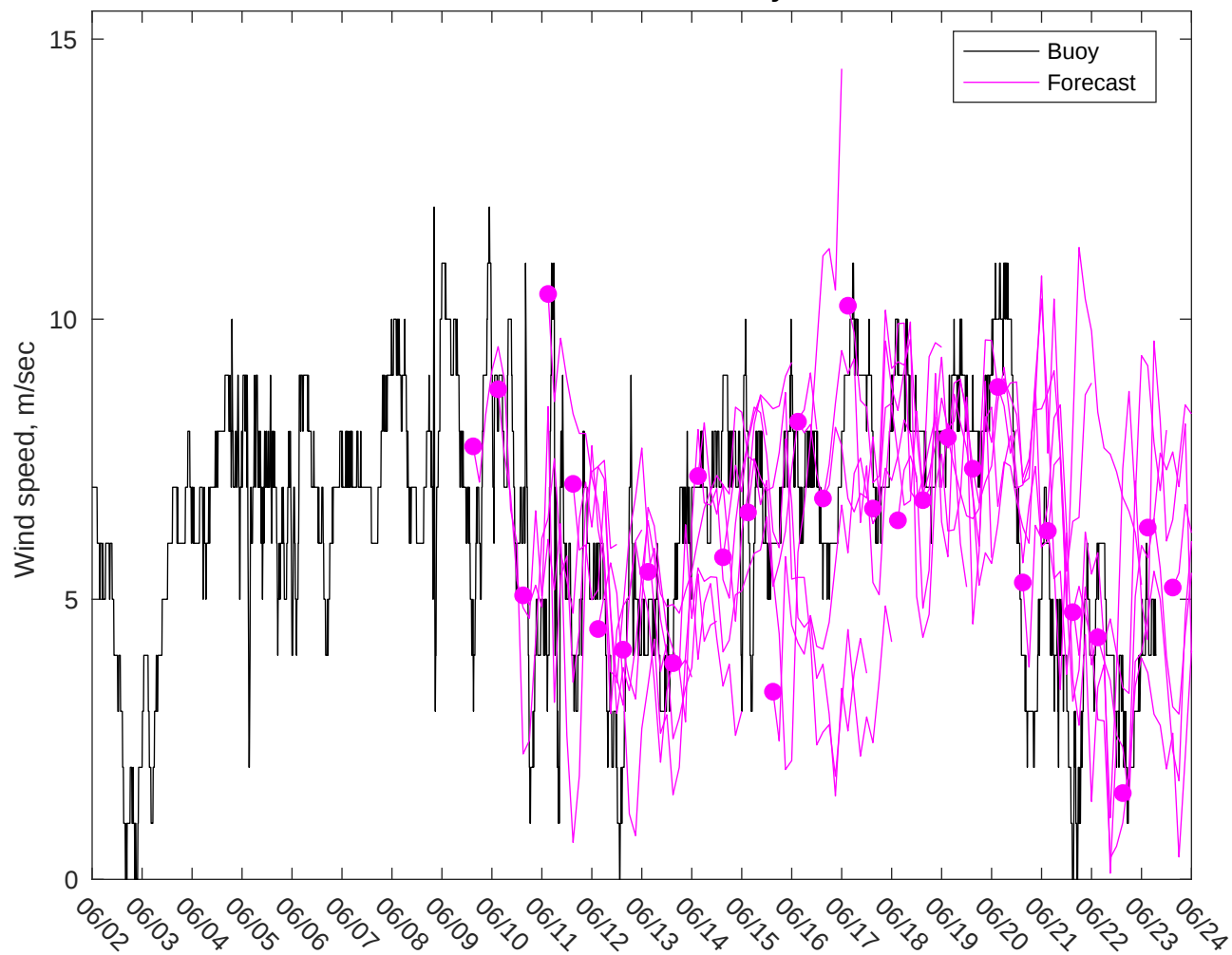
NDBC 41004 vs GFS Winds: 7 to 10 day forecast
