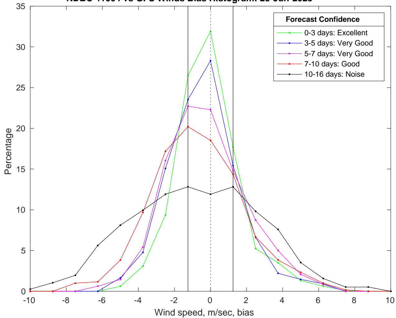
NDBC 41004 vs GFS Winds Bias Histogram: 23-Jun-2025
