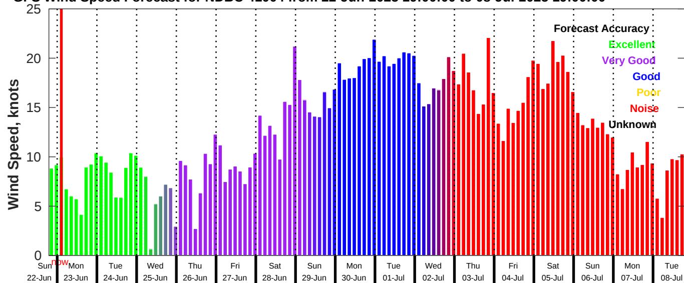
GFS Wind Speed Forecast for NDBC 41004 from 22-Jun-2025 19:00:00 to 08-Jul-2025 19:00:00
