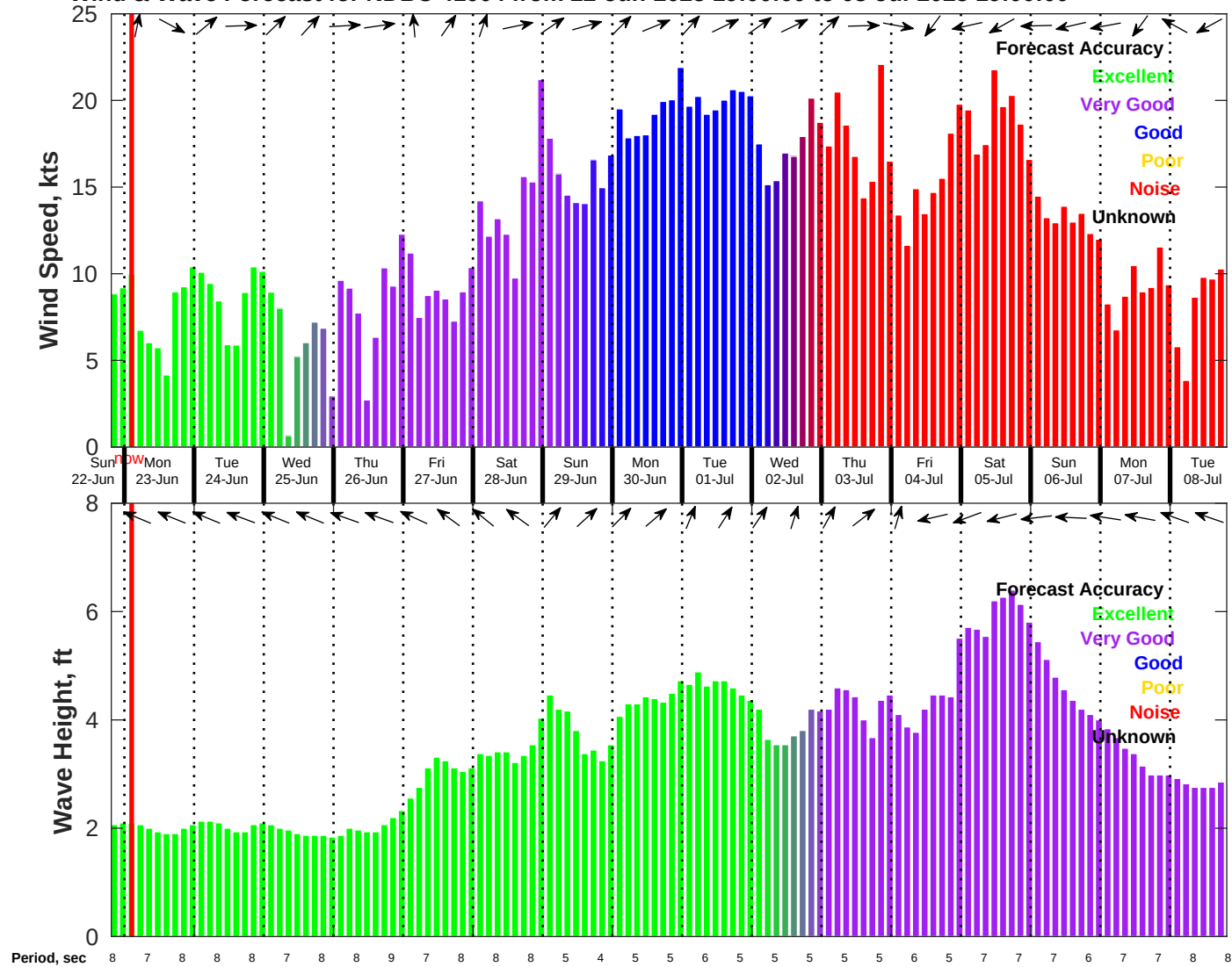
Wind & Wave Forecast for NDBC 41004 from 22-Jun-2025 19:00:00 to 08-Jul-2025 19:00:00
