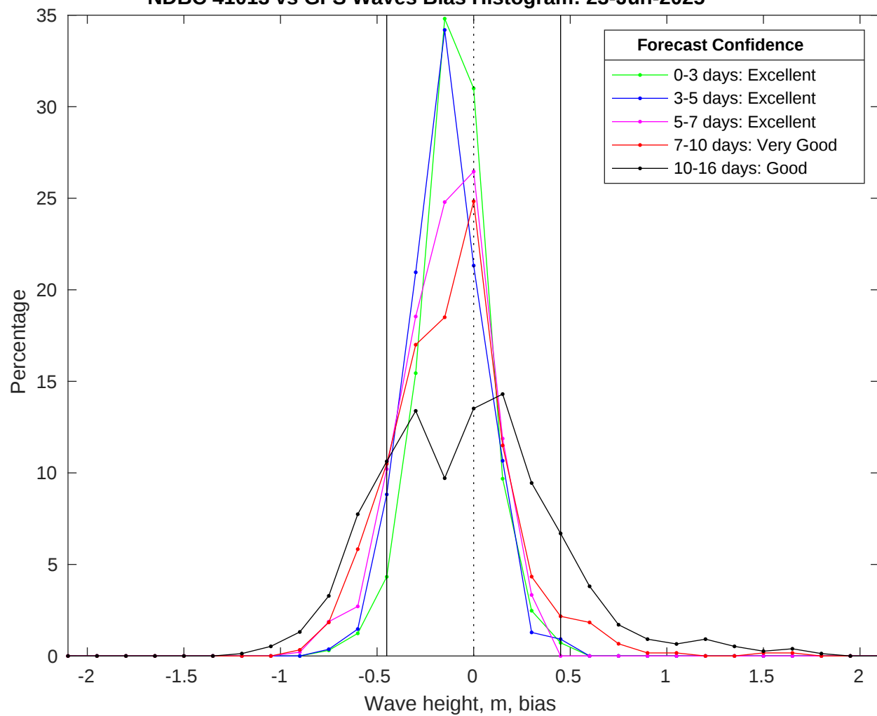
NDBC 41013 vs GFS Waves Bias Histogram: 23-Jun-2025
