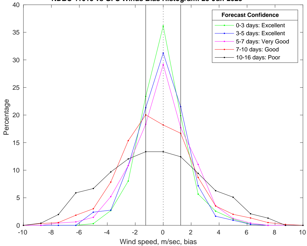
NDBC 41013 vs GFS Winds Bias Histogram: 23-Jun-2025
