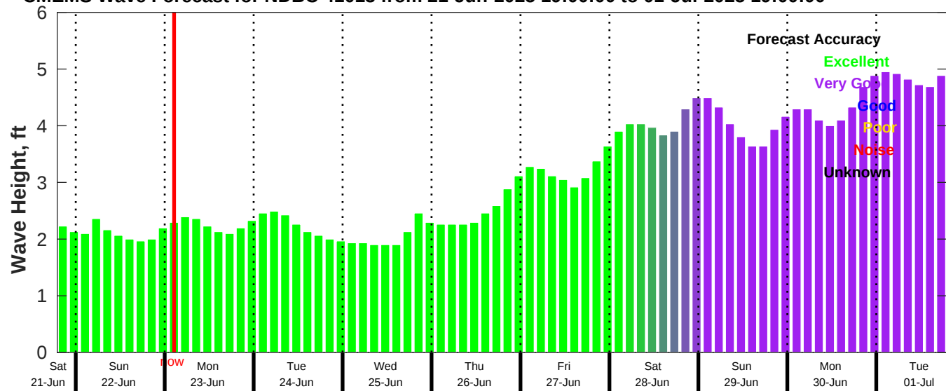
CMEMS Wave Forecast for NDBC 41013 from 21-Jun-2025 19:00:00 to 01-Jul-2025 19:00:00
