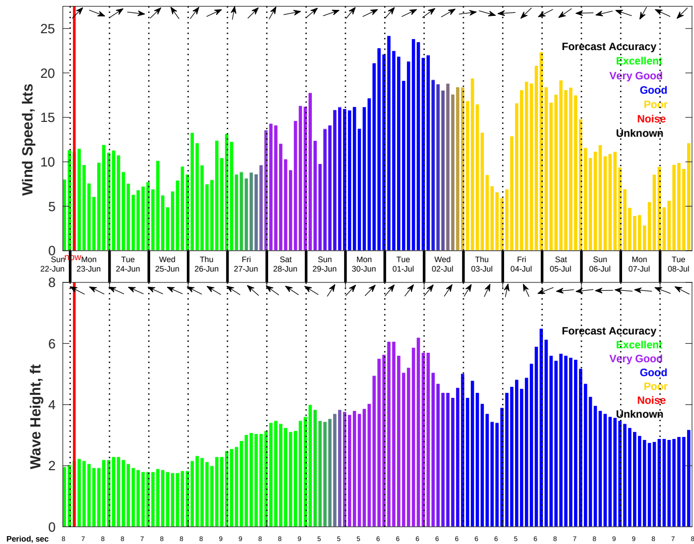
Wind & Wave Forecast for NDBC 41013 from 22-Jun-2025 19:00:00 to 08-Jul-2025 19:00:00
