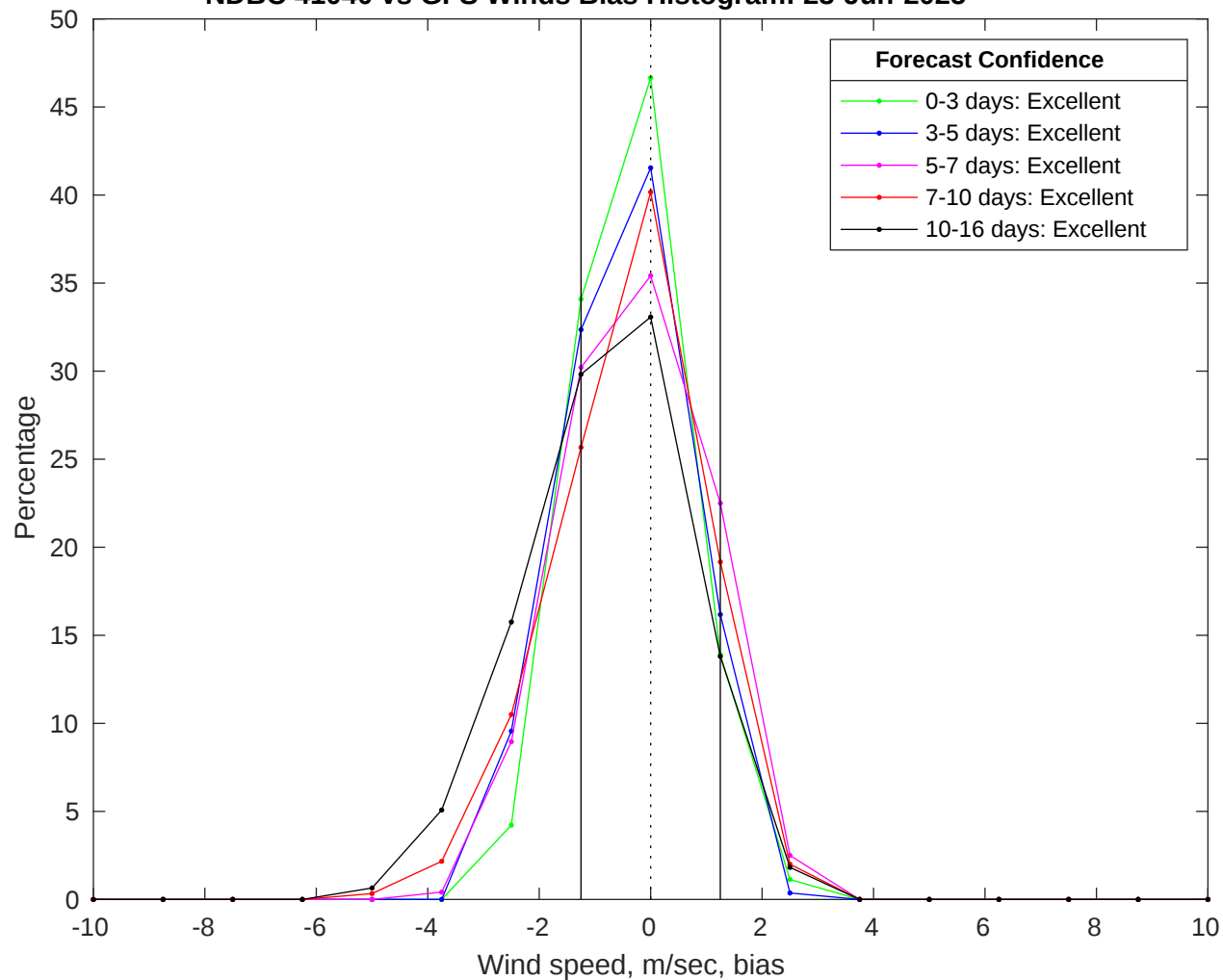
NDBC 41040 vs GFS Winds Bias Histogram: 23-Jun-2025
