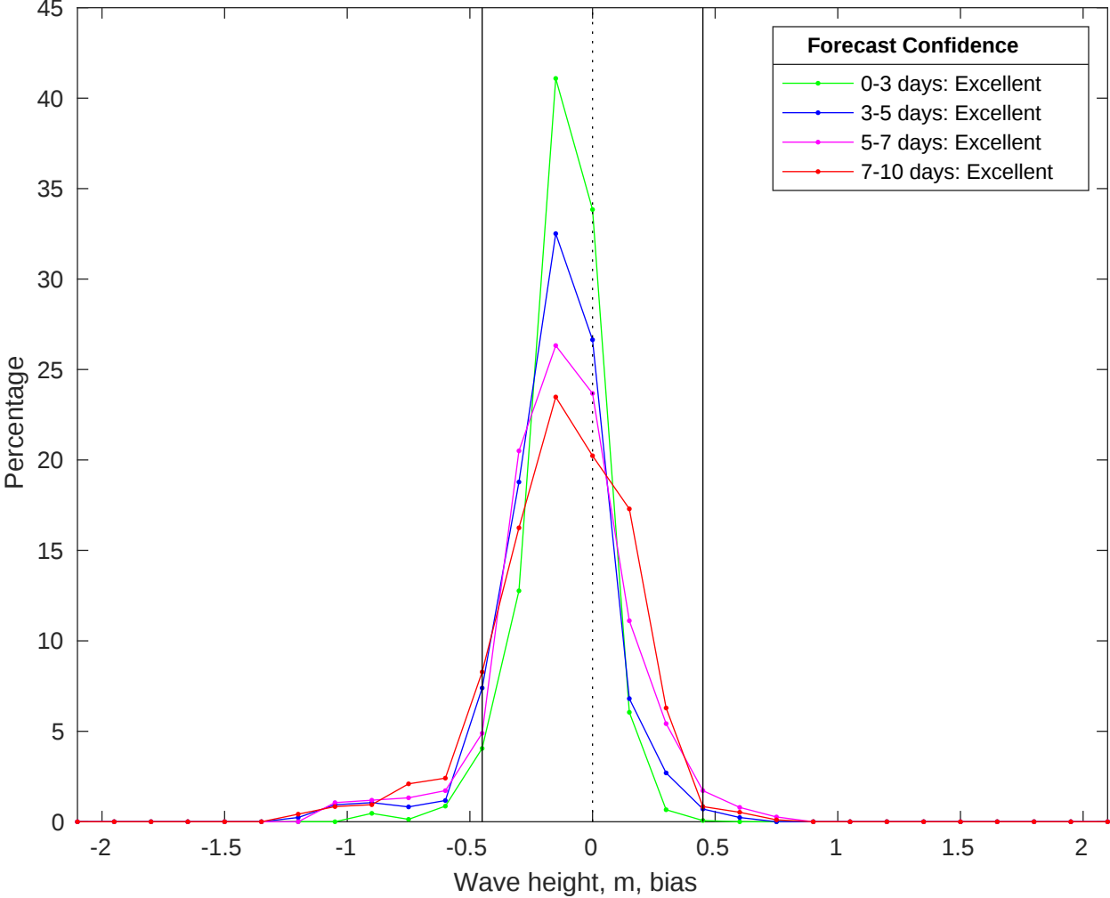
NDBC 42019 vs CMEMS Waves Bias Histogram: 23-Jun-2025
