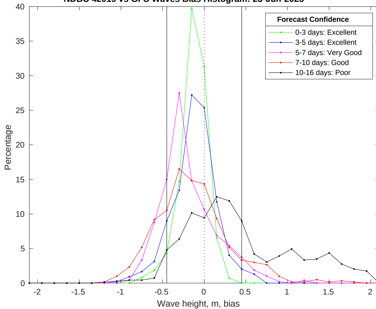
NDBC 42019 vs GFS Waves Bias Histogram: 23-Jun-2025
