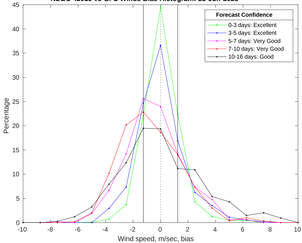
NDBC 42019 vs GFS Winds Bias Histogram: 23-Jun-2025
