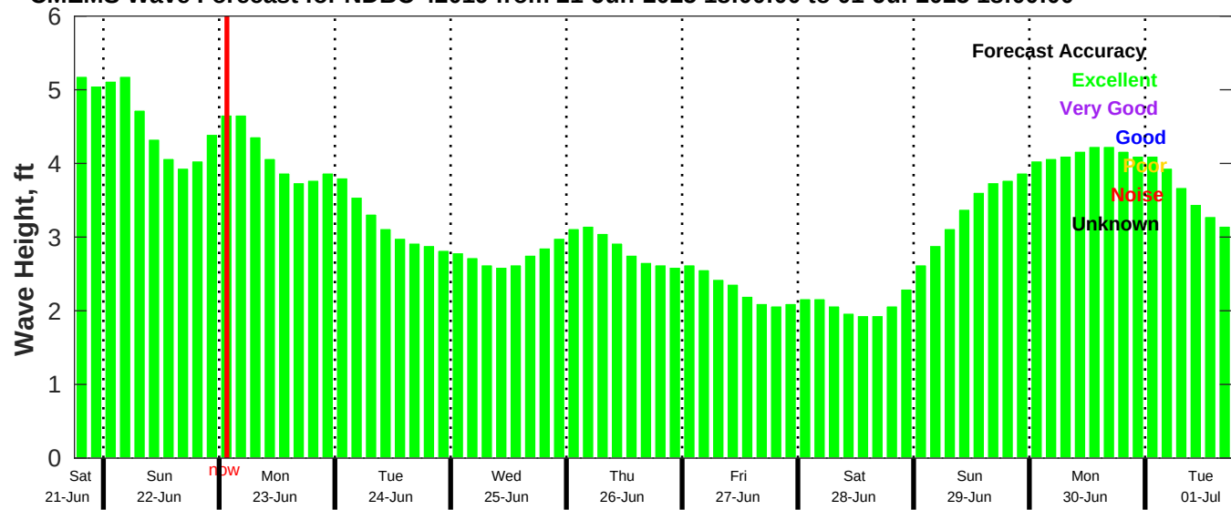
CMEMS Wave Forecast for NDBC 42019 from 21-Jun-2025 18:00:00 to 01-Jul-2025 18:00:00
