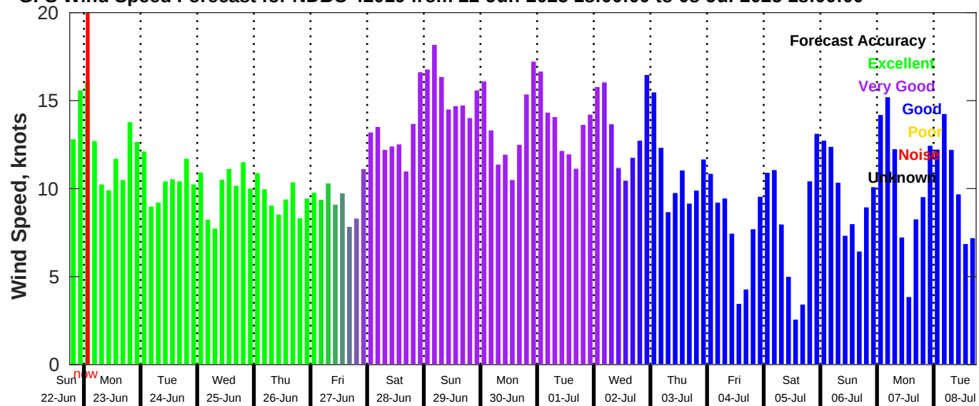
GFS Wind Speed Forecast for NDBC 42019 from 22-Jun-2025 18:00:00 to 08-Jul-2025 18:00:00
