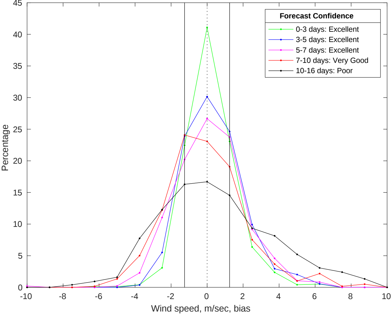
NDBC 42020 vs GFS Winds Bias Histogram: 23-Jun-2025
