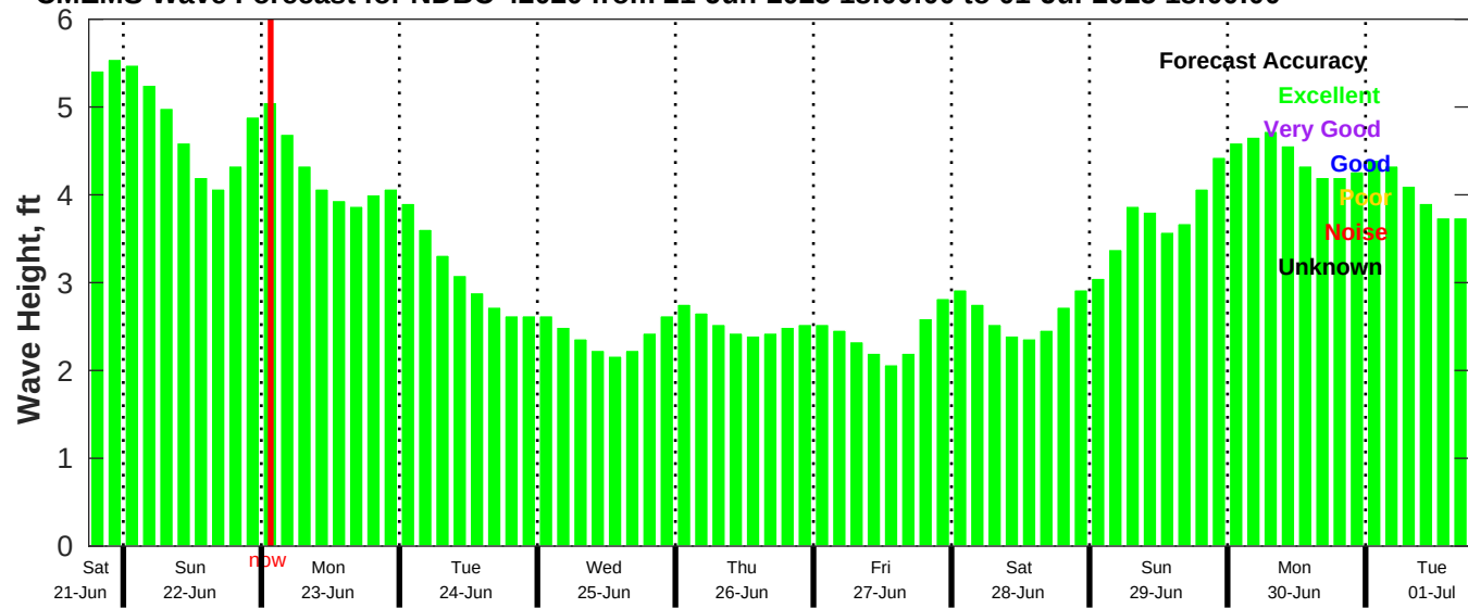
CMEMS Wave Forecast for NDBC 42020 from 21-Jun-2025 18:00:00 to 01-Jul-2025 18:00:00
