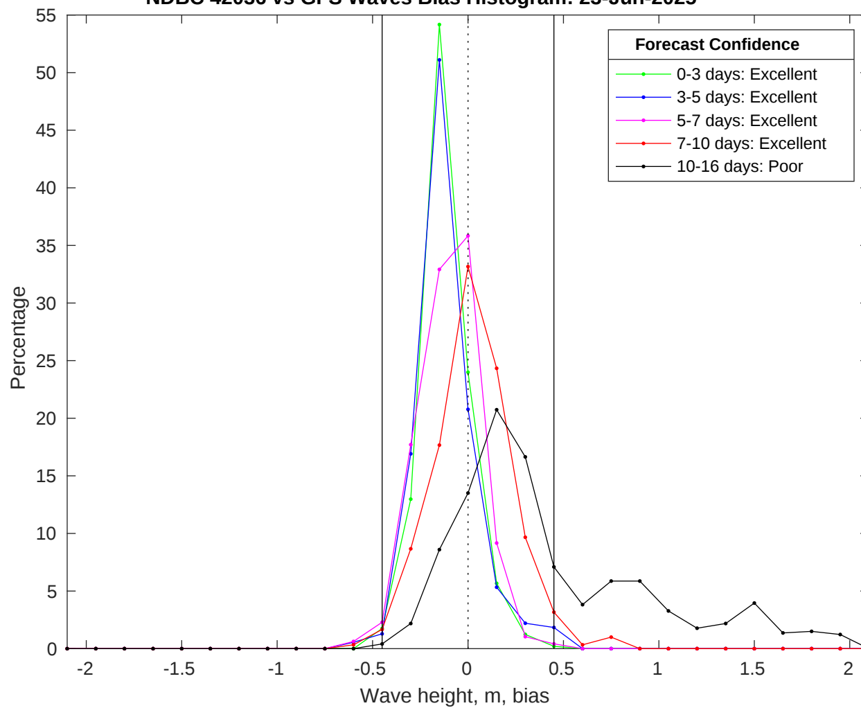
NDBC 42036 vs GFS Waves Bias Histogram: 23-Jun-2025
