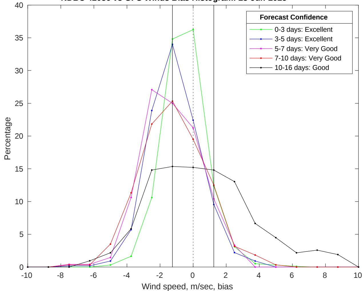
NDBC 42036 vs GFS Winds Bias Histogram: 23-Jun-2025
