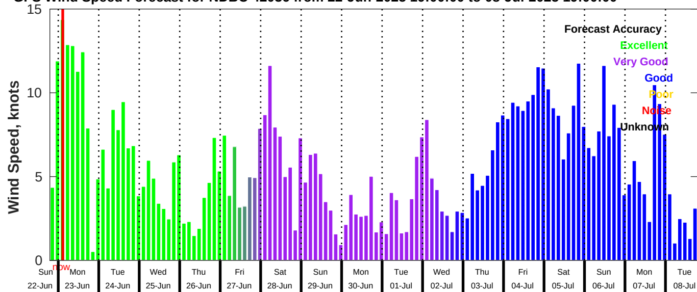
GFS Wind Speed Forecast for NDBC 42036 from 22-Jun-2025 19:00:00 to 08-Jul-2025 19:00:00
