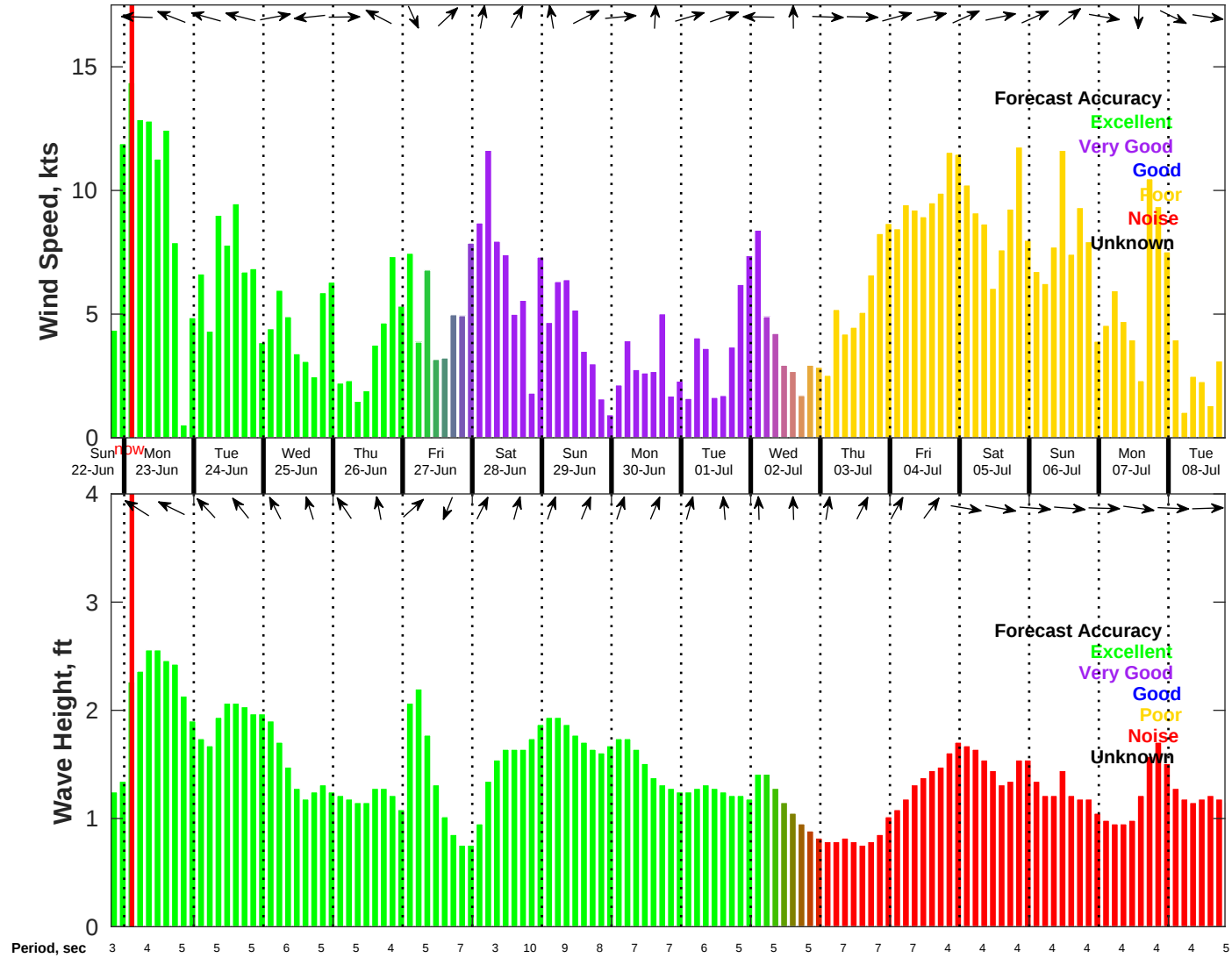
Wind & Wave Forecast for NDBC 42036 from 22-Jun-2025 19:00:00 to 08-Jul-2025 19:00:00
