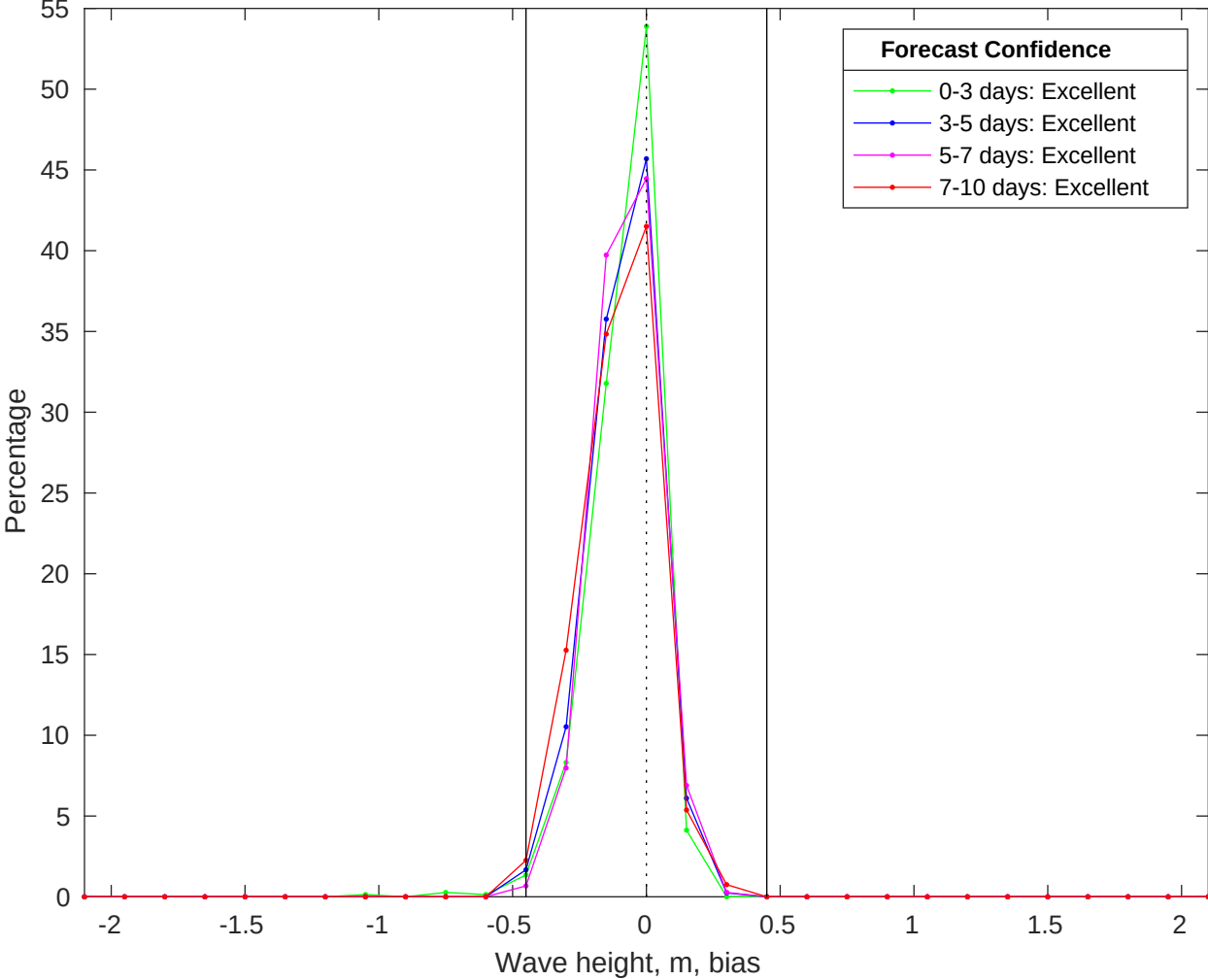
NDBC 42040 vs CMEMS Waves Bias Histogram: 23-Jun-2025
