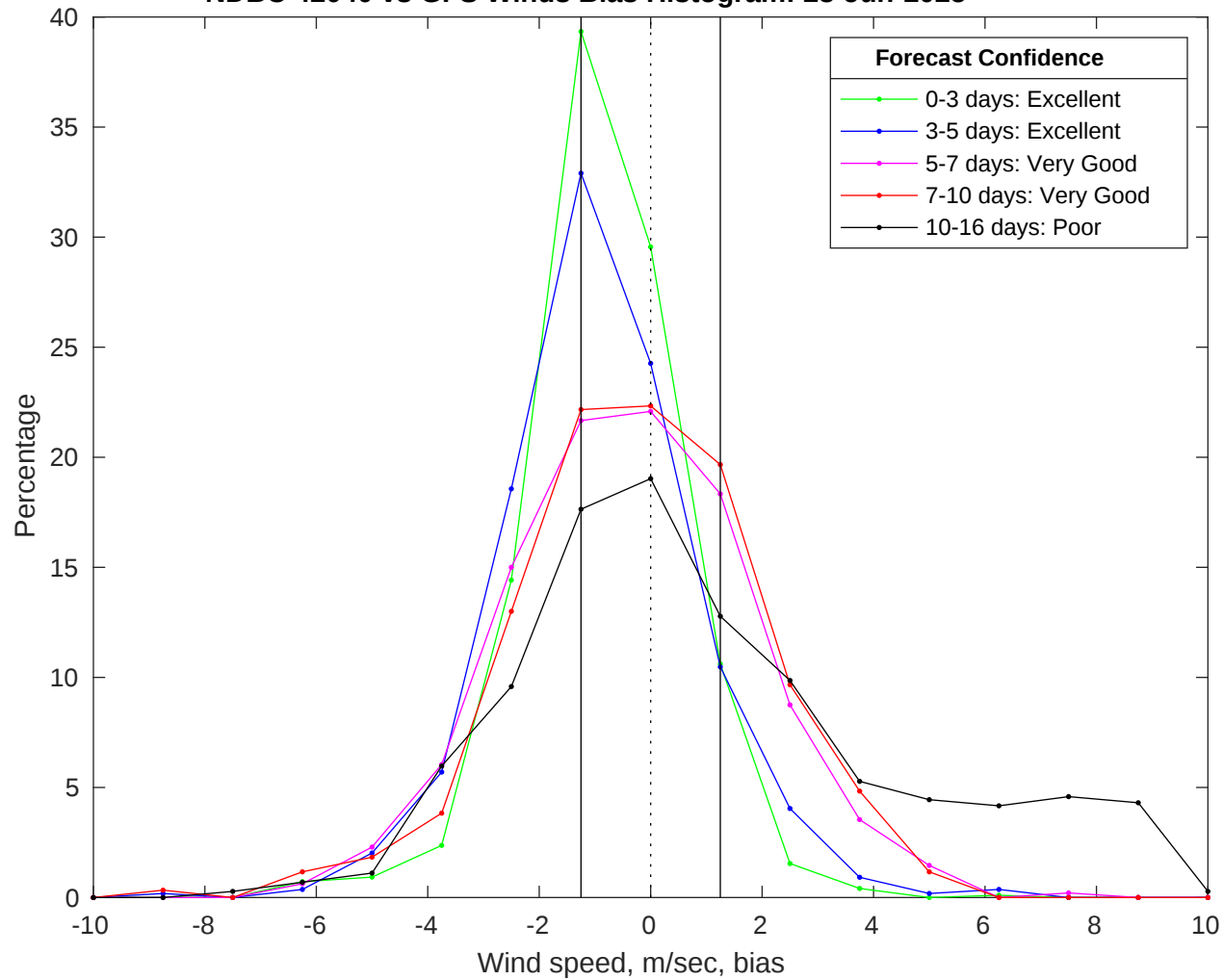
NDBC 42040 vs GFS Winds Bias Histogram: 23-Jun-2025
