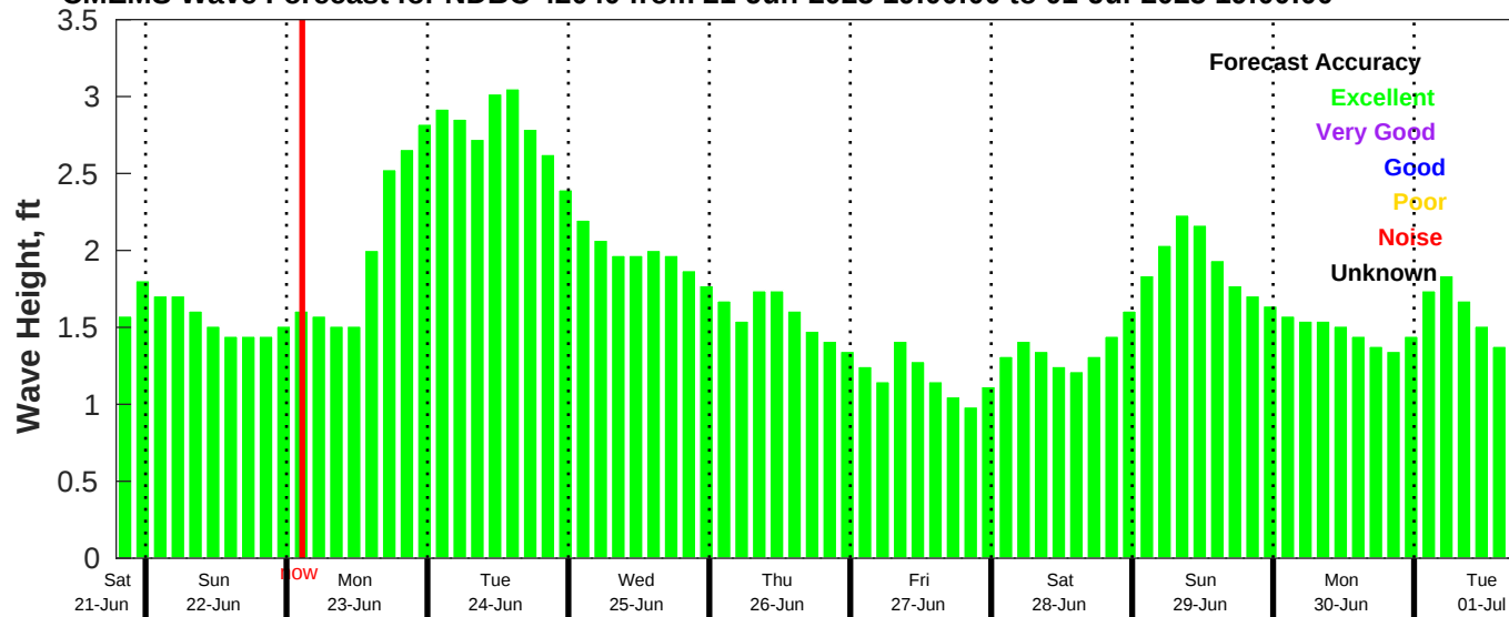
CMEMS Wave Forecast for NDBC 42040 from 21-Jun-2025 19:00:00 to 01-Jul-2025 19:00:00
