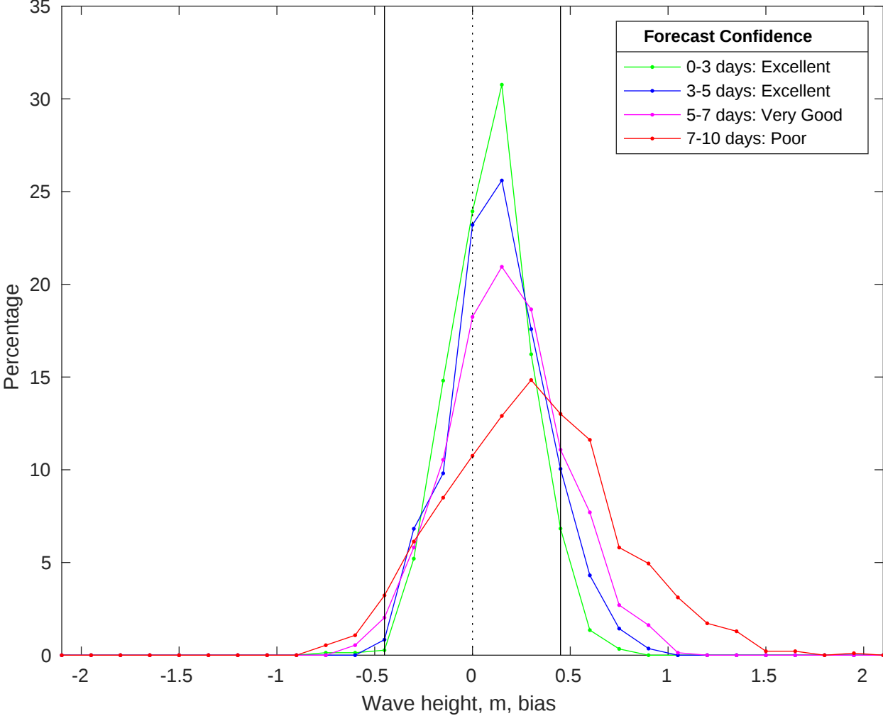
NDBC 46011 vs CMEMS Waves Bias Histogram: 23-Jun-2025
