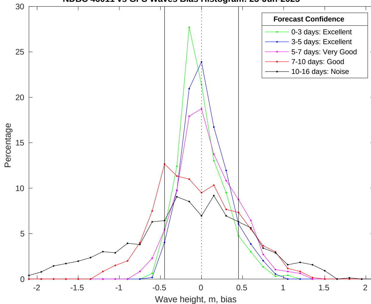
NDBC 46011 vs GFS Waves Bias Histogram: 23-Jun-2025
