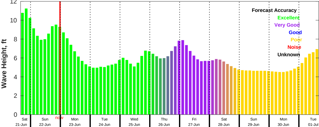
CMEMS Wave Forecast for NDBC 46011 from 21-Jun-2025 16:00:00 to 01-Jul-2025 16:00:00
