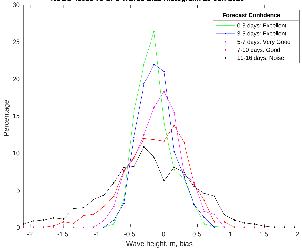
NDBC 46028 vs GFS Waves Bias Histogram: 23-Jun-2025
