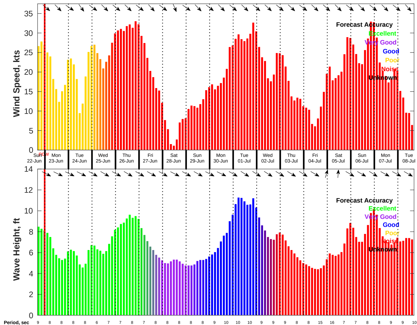
Wind & Wave Forecast for NDBC 46028 from 22-Jun-2025 16:00:00 to 08-Jul-2025 16:00:00
