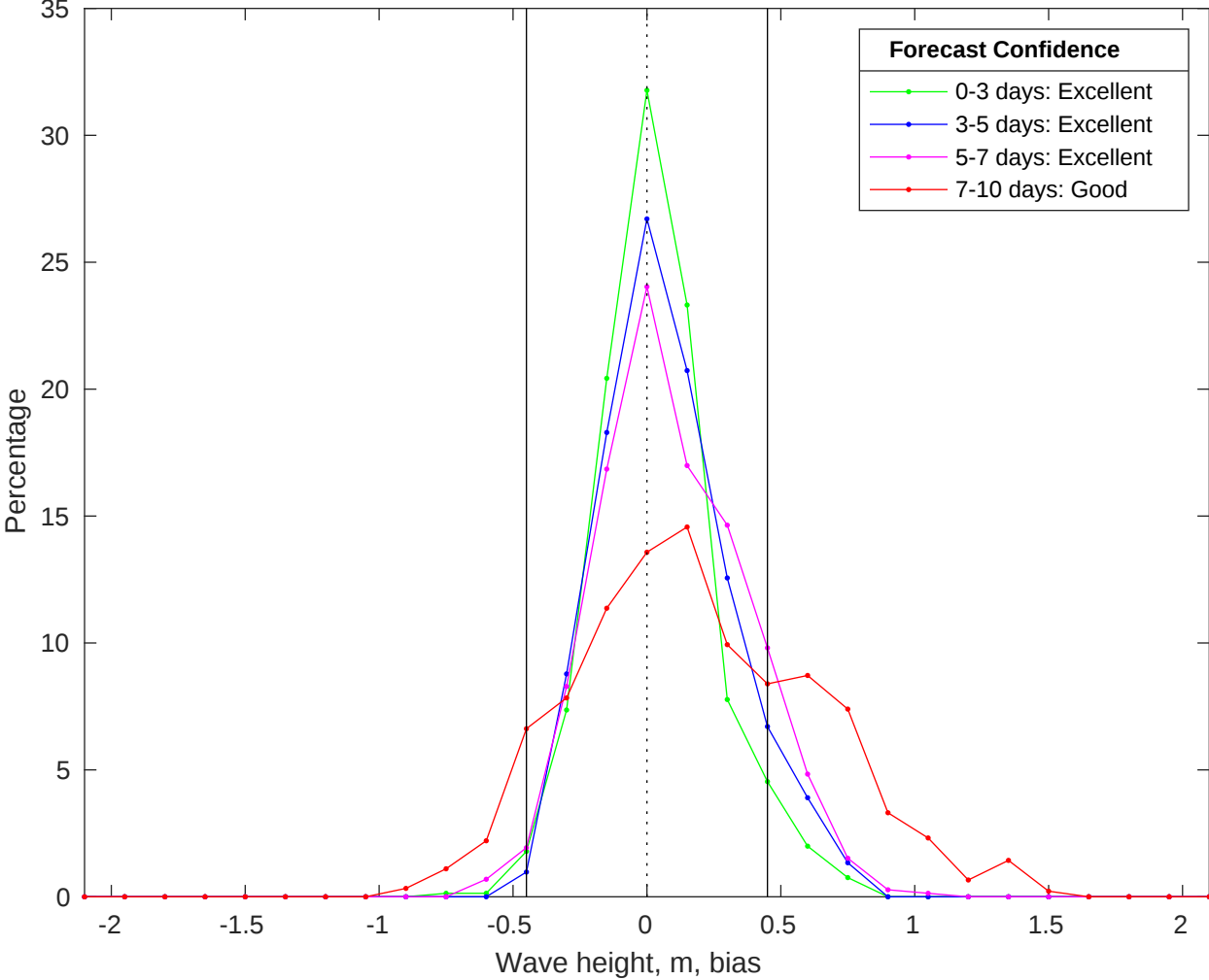
NDBC 46054 vs CMEMS Waves Bias Histogram: 23-Jun-2025
