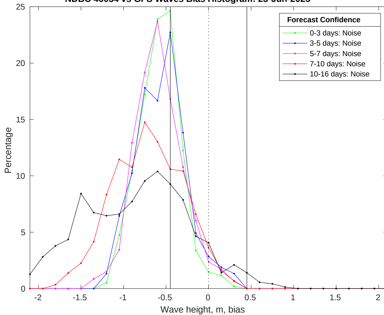
NDBC 46054 vs GFS Waves Bias Histogram: 23-Jun-2025
