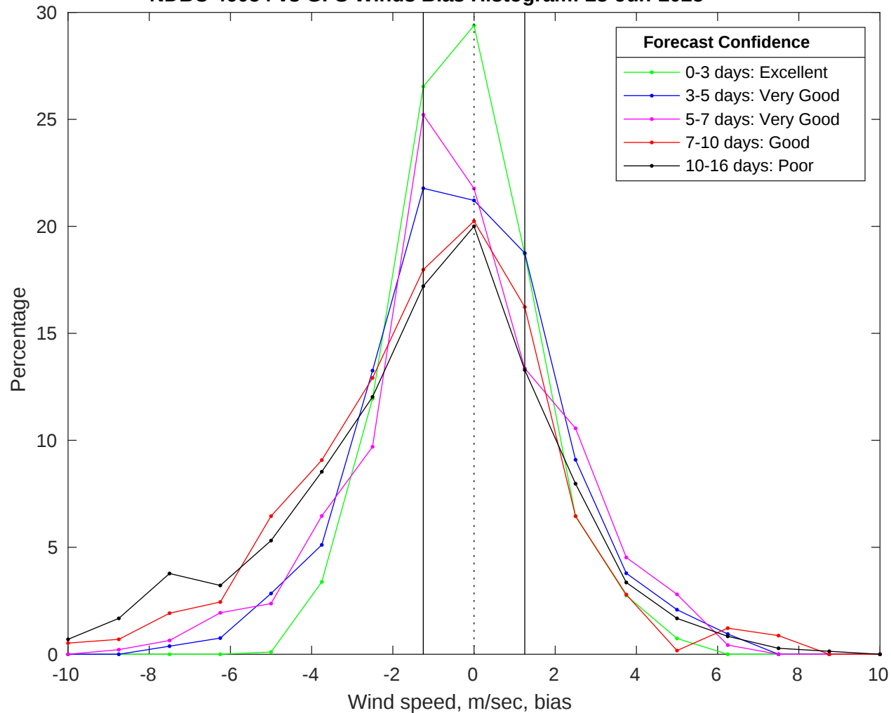
NDBC 46054 vs GFS Winds Bias Histogram: 23-Jun-2025
