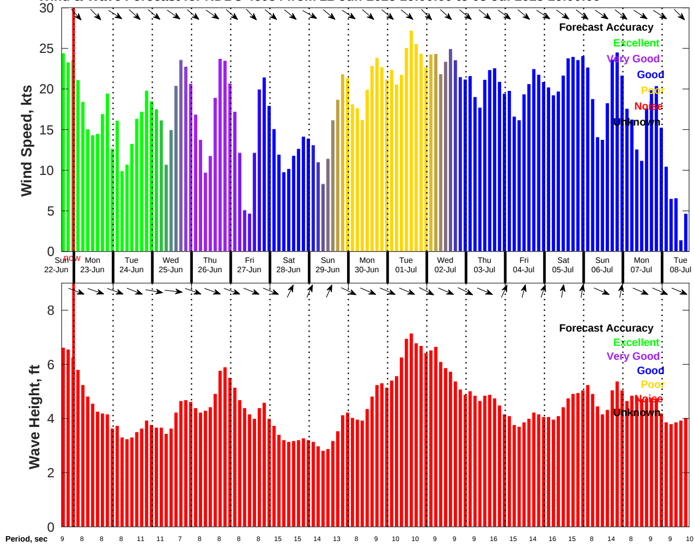
Wind & Wave Forecast for NDBC 46054 from 22-Jun-2025 16:00:00 to 08-Jul-2025 16:00:00
