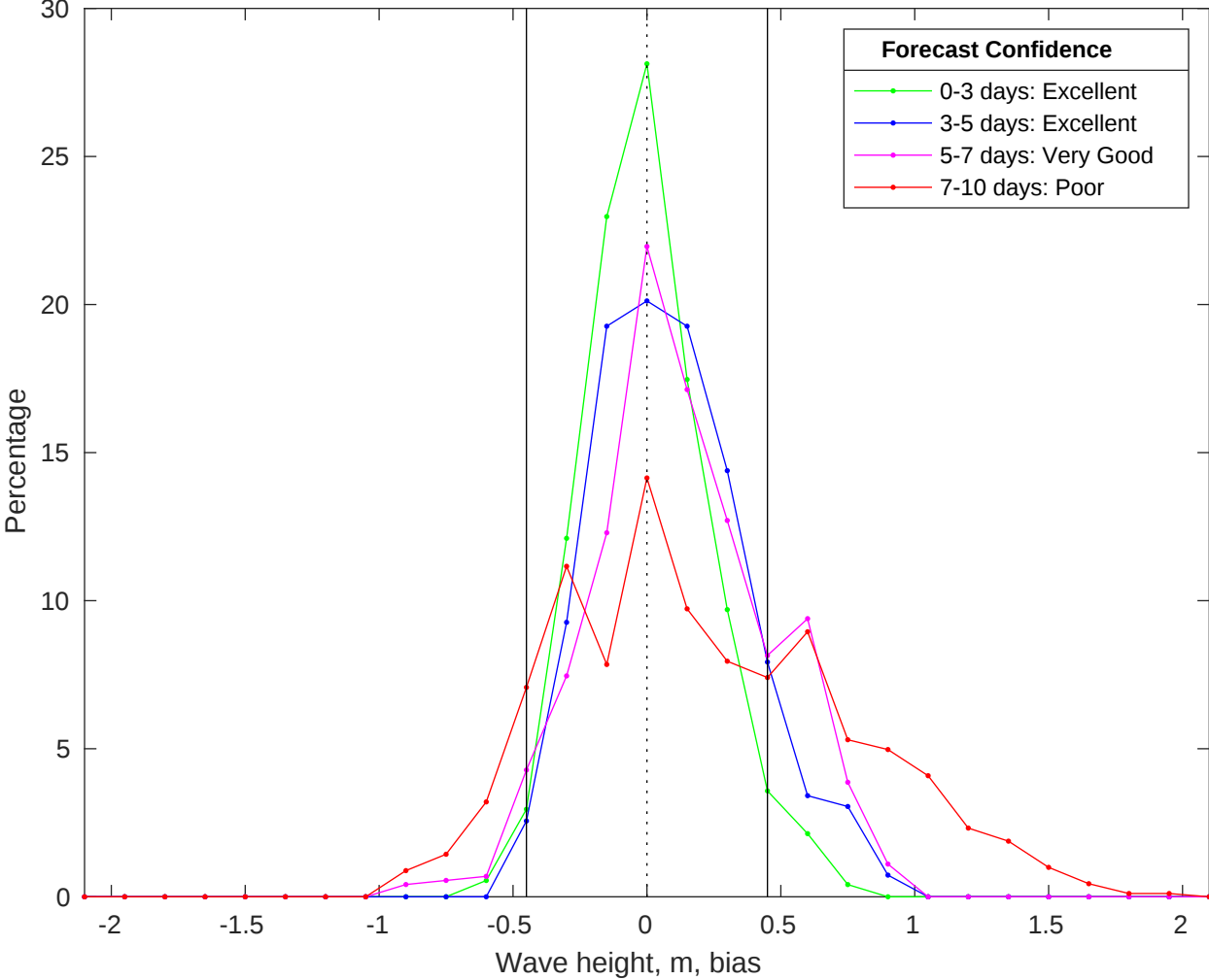
NDBC 46069 vs CMEMS Waves Bias Histogram: 23-Jun-2025
