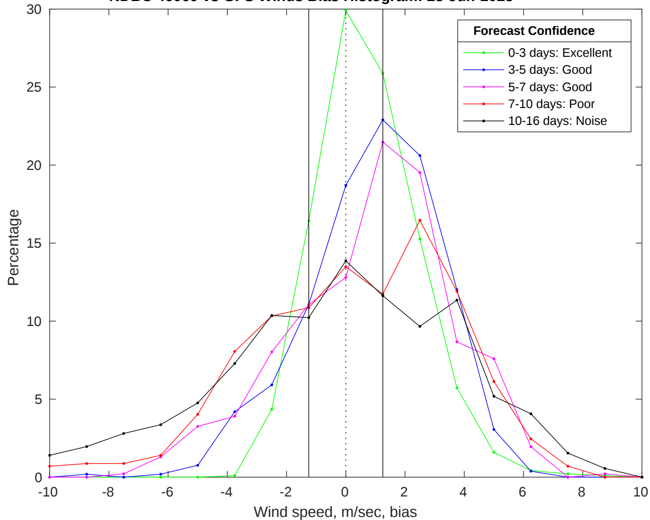
NDBC 46069 vs GFS Winds Bias Histogram: 23-Jun-2025
