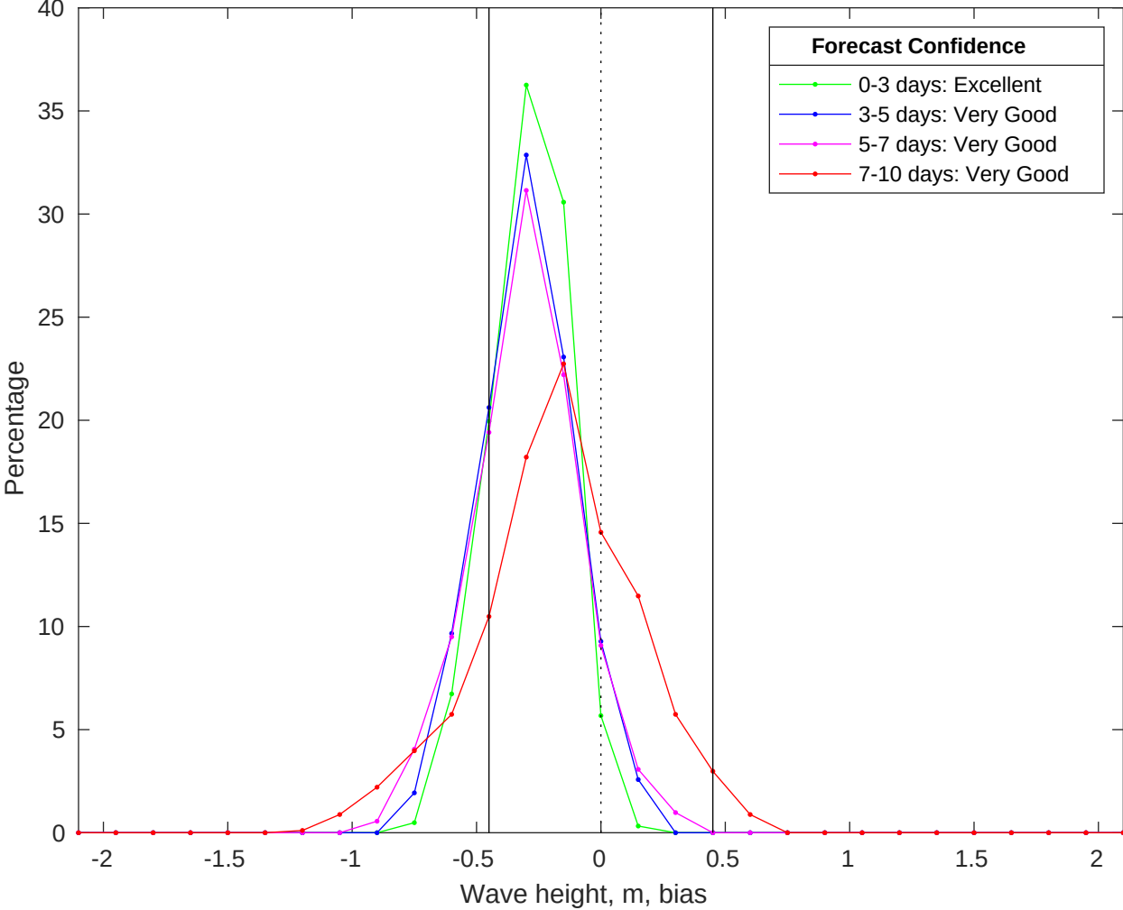
NDBC 51209 vs CMEMS Waves Bias Histogram: 23-Jun-2025
