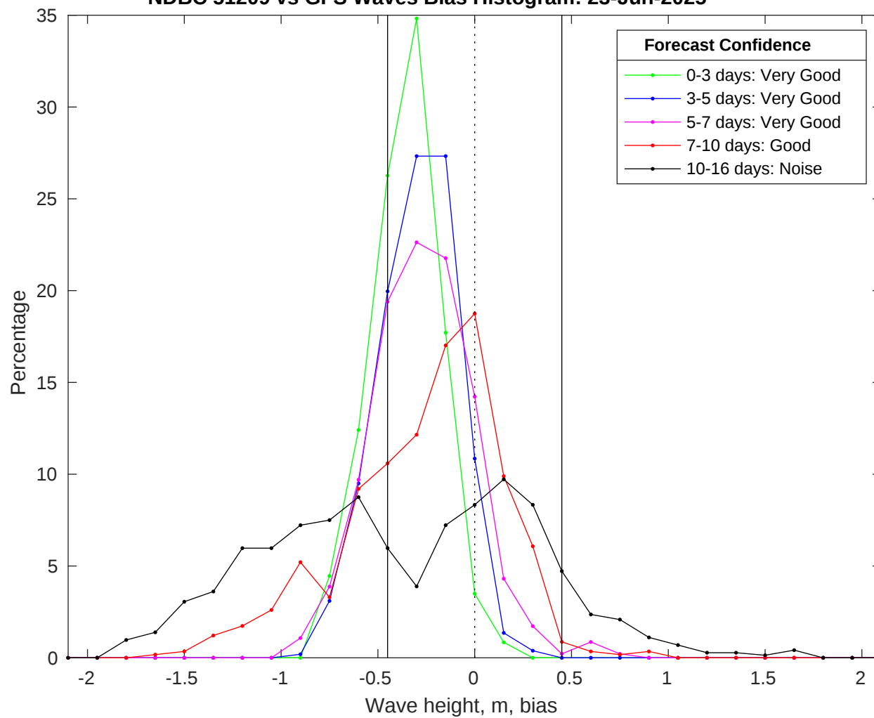
NDBC 51209 vs GFS Waves Bias Histogram: 23-Jun-2025
