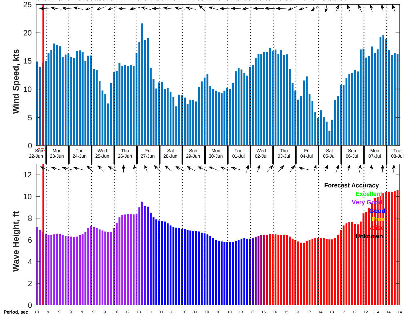
Wind & Wave Forecast for NDBC 51209 from 22-Jun-2025 13:00:00 to 08-Jul-2025 13:00:00
